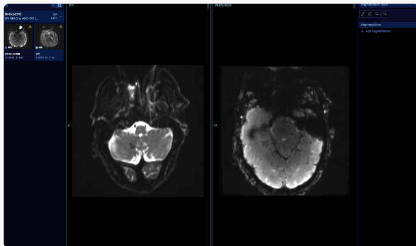
DICOM Viewer
